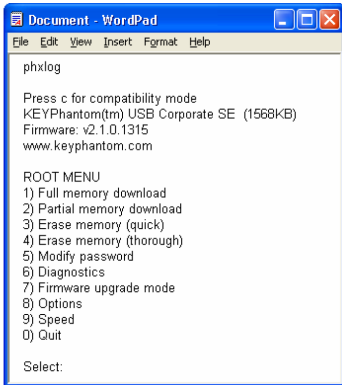
Figure 4 - KeyCarbon™ USB menu.
