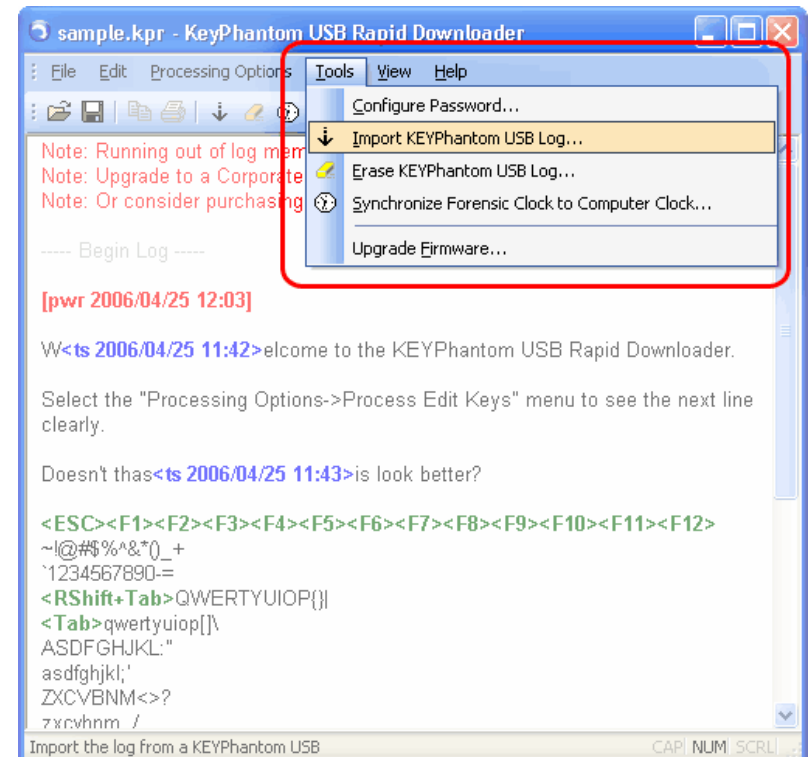
Figure 2 - KeyCarbon™ USB Rapid Downloader utility.
